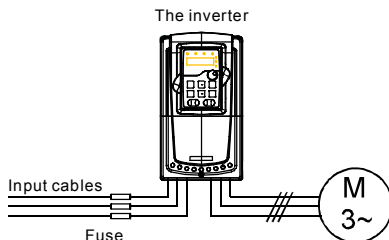
Fig 4-25 Fuse configuration
